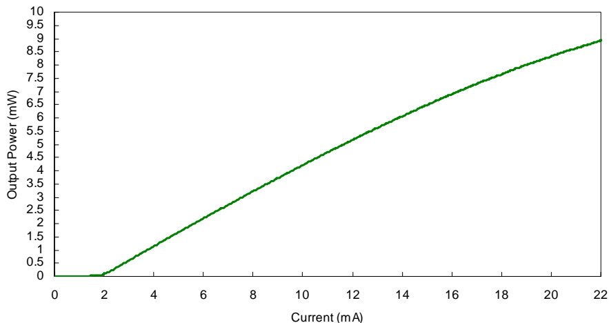
Fig .2 Typical Electrical Characteristics
