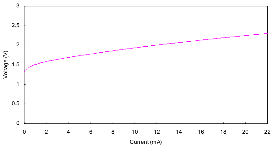
Typical Voltage vs Current
