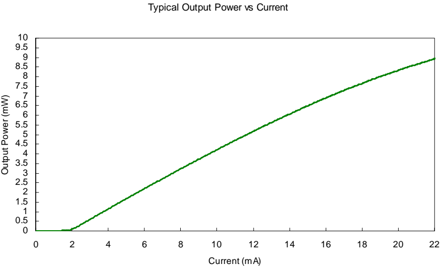
Fig .1 Typical Optical Characteristics
