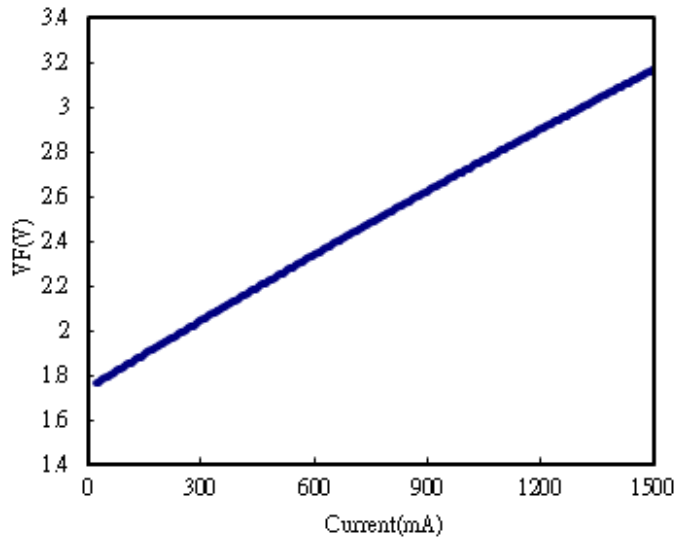
Fig.4 The V-I characteristics (0-1500mA)
