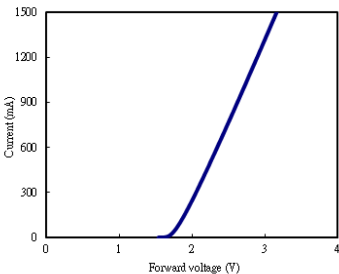
Fig.1 The I-V characteristics (0-1500mA)
