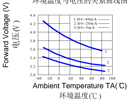
Forward Voltage Derating Curve 环境温度与电压的关系曲线图
