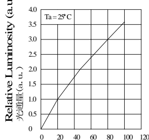
Forward Current IFP (mA) 电流 (mA)
