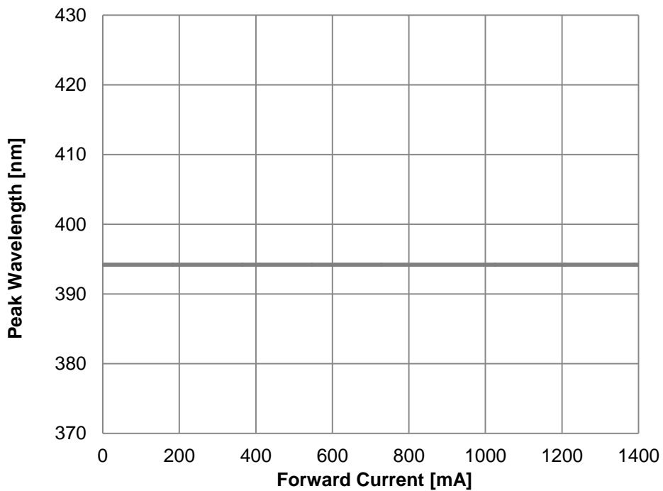
Fig 4. Forward Current vs. Peak Wavelength, T_a=25^\circ\text{C}
