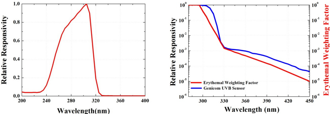
Figure9.2Spectral Responsivity Characteristics
