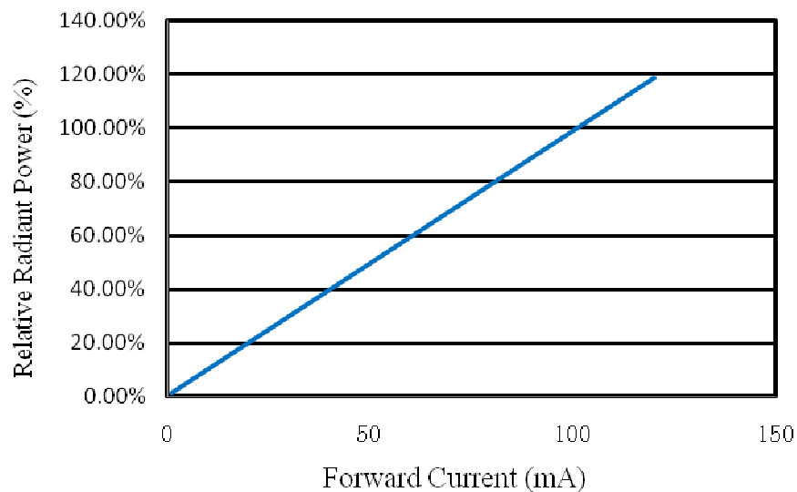
Relative Radiant Power VS Forward Current (Ta=25 °C)
