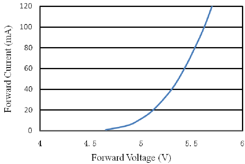
Forward Current VS Forward Voltage (Ta=25 °C)
