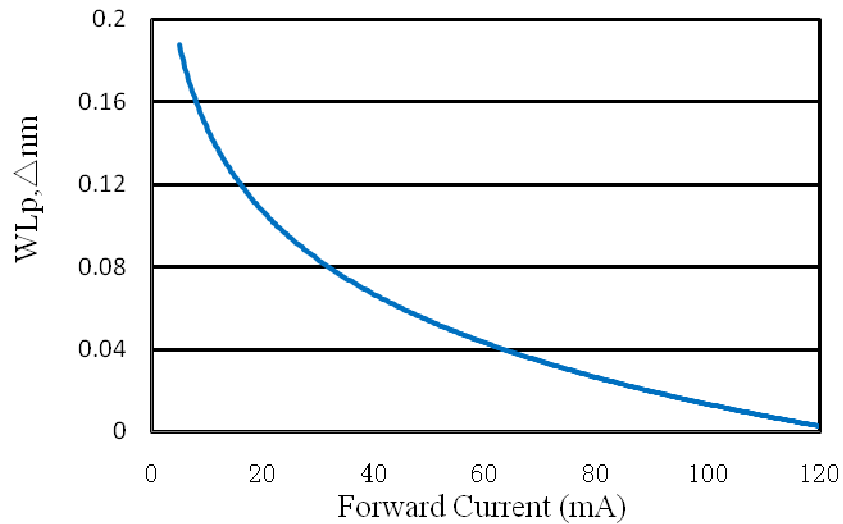
Wavelength \Delta Vs Forward Current (Ta=25°C)
