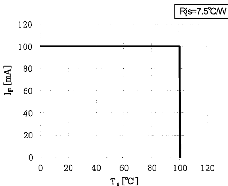
Allowed area to operate: I_F - T_s
