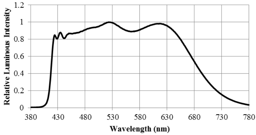
Spectrum (Ta=25 , If=65mA)
