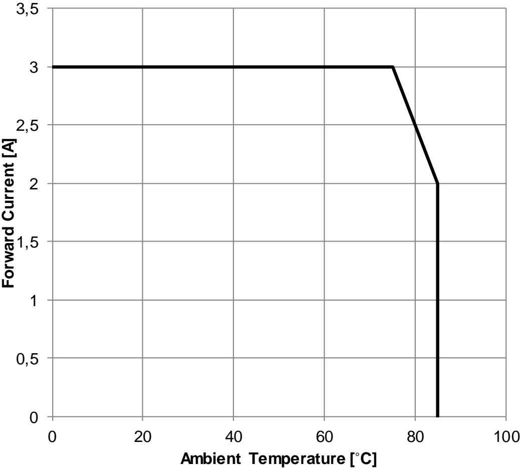
Derating Curve:
