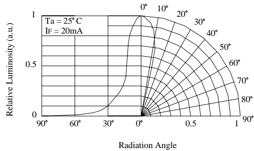
Directivity ( Angle : 25° )
